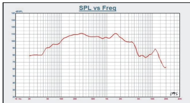
LA-1200P SPL VS Frequency Response
